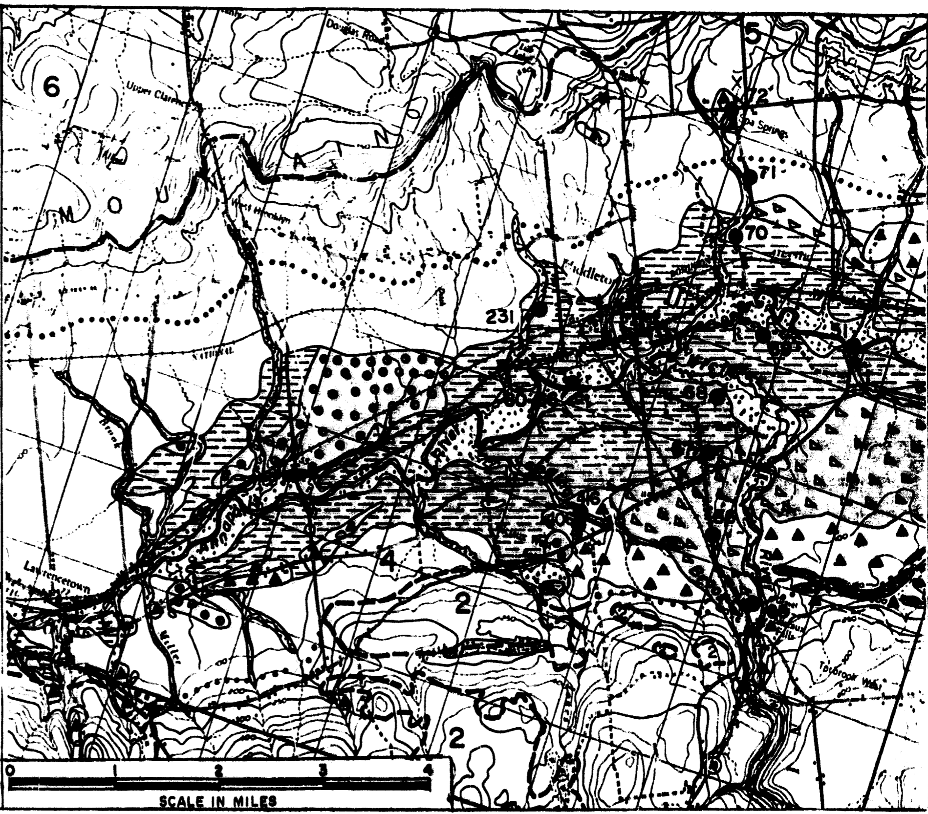
FIGURE 2. General geology of the Nictaux West - Middleton area.
