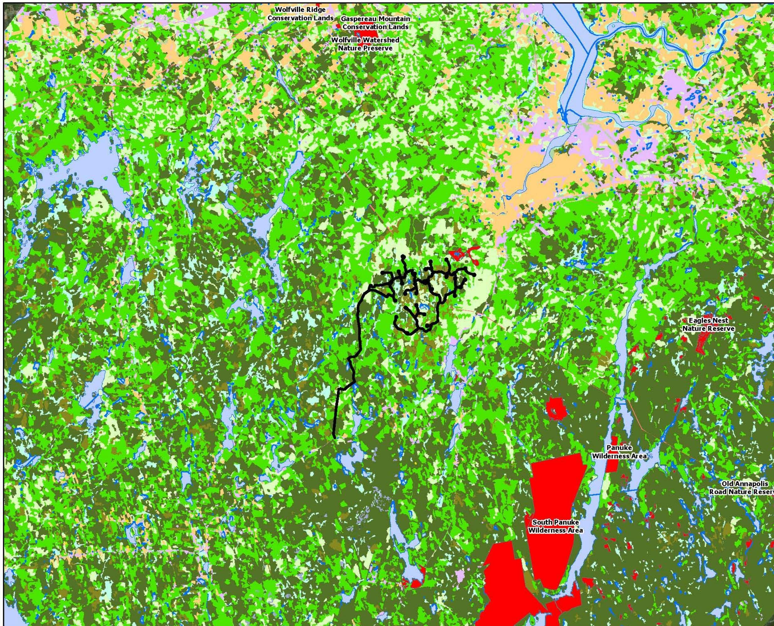
Figure 21 Land Cover Types within Project Region
